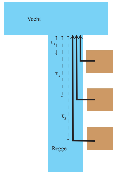
Figure 3.6: Sketch of subcatchments with a different distance to the Vecht, leading to a time lag \tau_i in the time when the water reaches the Vecht.
