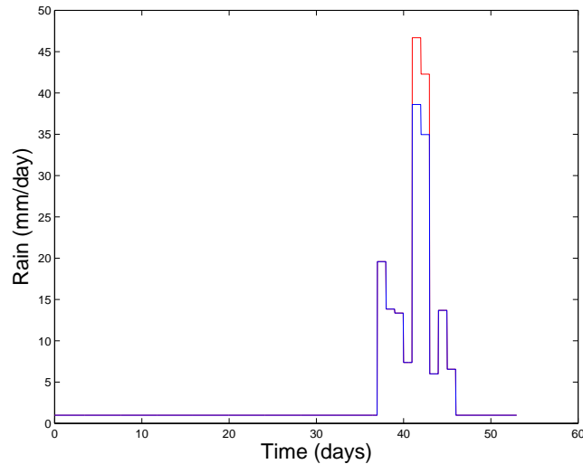
Figure 3.2: Benchmark precipitation event before (blue) and after (red) after climate change.
