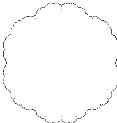
Figure 4. The limit case of figure 3. The centre of the picture is 0, the six dots nearest to 0 are the elements \pm 1, \pm\rho, \pm\rho^2 of the ring. For \alpha in \mathbb{Z}[\rho] , \alpha \neq 0 , we have \psi(\alpha) < n if and only if \alpha(1 - \rho)^{-n} is inside the dodecagonal figure, but not equal to one of the dots. The intersection of the closure of the set and the boundary of its convex hull consists of twelve copies of the Cantor discontinuum.
