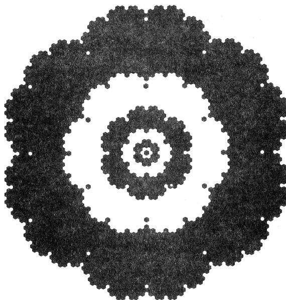
Figure 3. The smallest division algorithm on the ring \mathbb{Z}[\rho] = \{a + b\rho : a \text{ and } b \text{ are integers}\} , where \rho = (-1 + \sqrt{-3})/2 is a primitive cube root of unity. The ring is a triangular lattice in the complex plane, and the points of the lattice are the centers of a regular hexagonal tiling of the plane. The black hexagons in the picture correspond to the elements \alpha of \mathbb{Z}[\rho] for which \alpha = 0 or \psi(\alpha) = 1, 3 or 5 .
