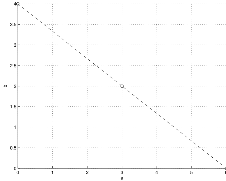
Figure 4.1: Example 1: Support of f(x, y) = y^4 - 2x^3y^2 + x^6
