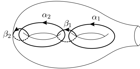
Figure 5.6: Vanishing cycles on disk
